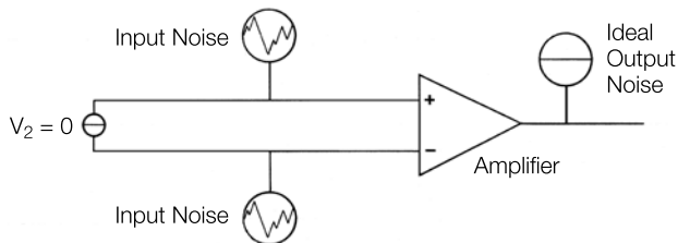
Figure 4. Noise cancellation by amplifier common-mode rejection.
